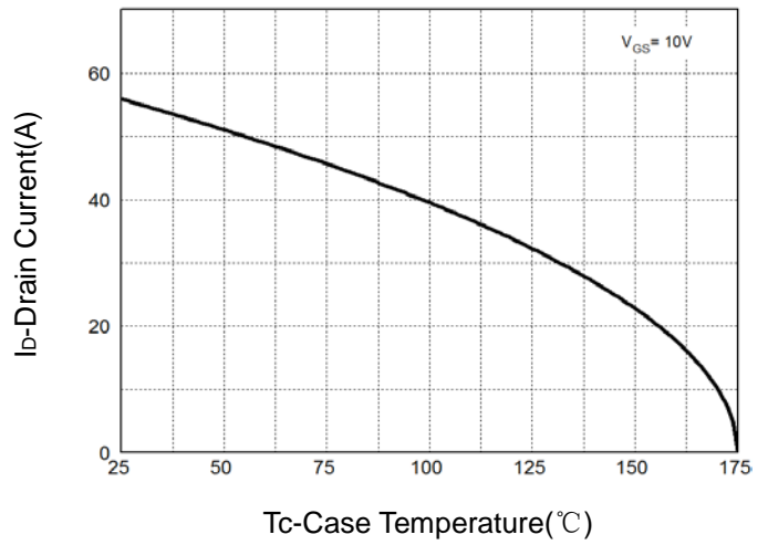
Figure 2: Drain Current
